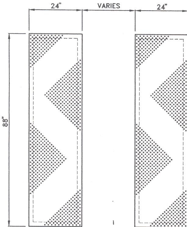
PANEL ELEVATION
