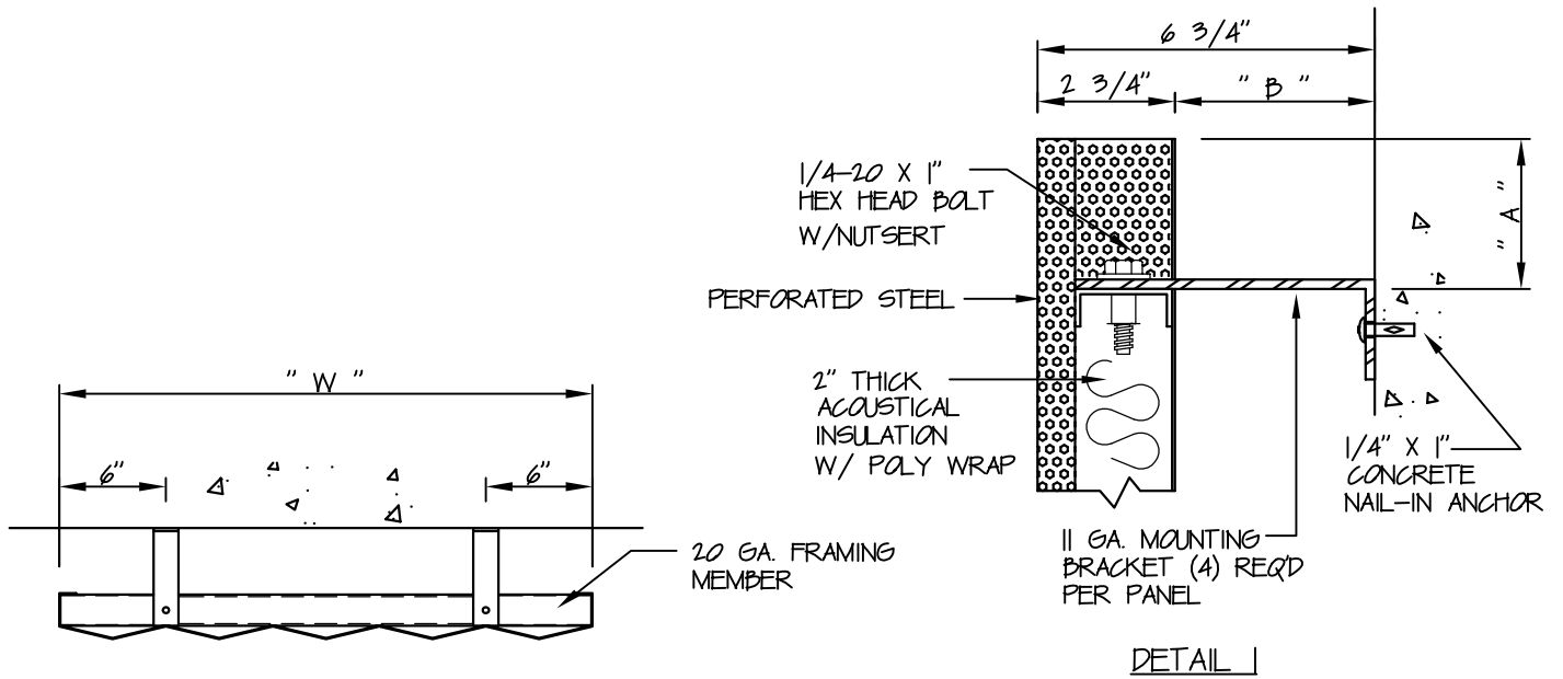
CROSS SECTION
