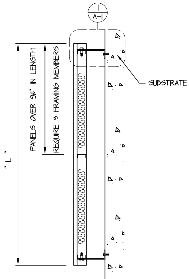
VERTICAL SECTION
